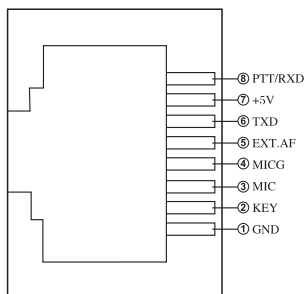
Microphone plug (view from the front)
